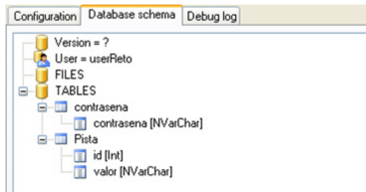
Figure 15: Marathon Tool Database Schema
