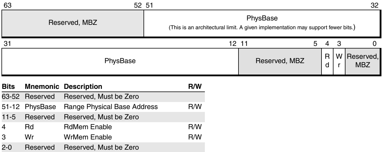
Figure 7-12. IORRBase_n Register
