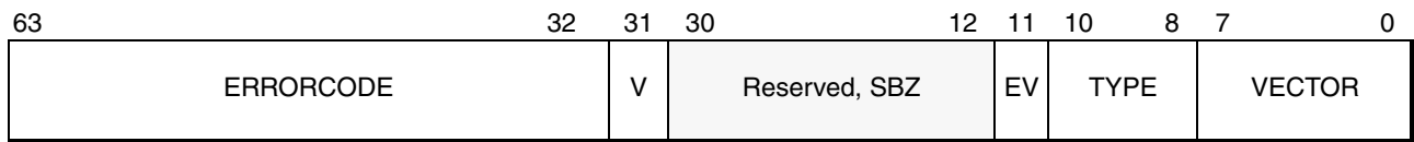
Figure 15-4. EVENTINJ Field in the VMCB
