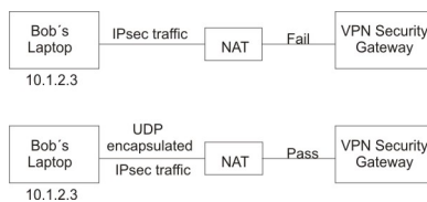
Figure 12. NAT-enabled IP Security
