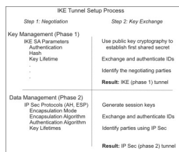
Figure 9. IKE Tunnel Setup Process
